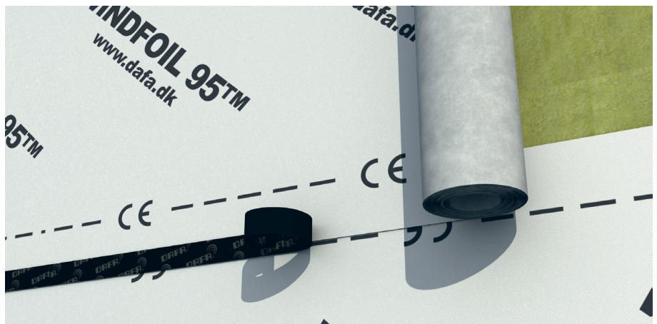
DAFA WindFoil 95 is installed as a wind barrier with a minimum overlap of 150 mm and free joints are taped using DAFA UV tape.
