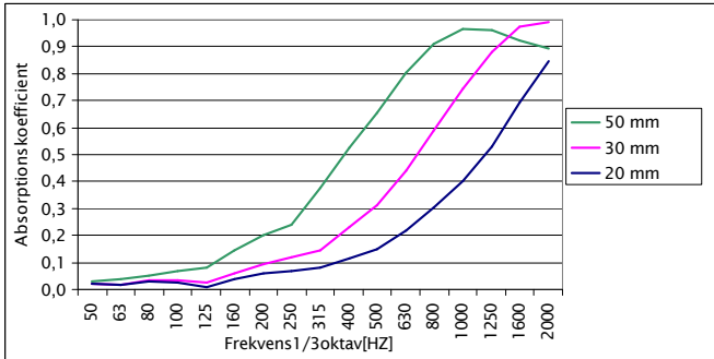
Sound absorption, a [%] according to ISO 10534-2
