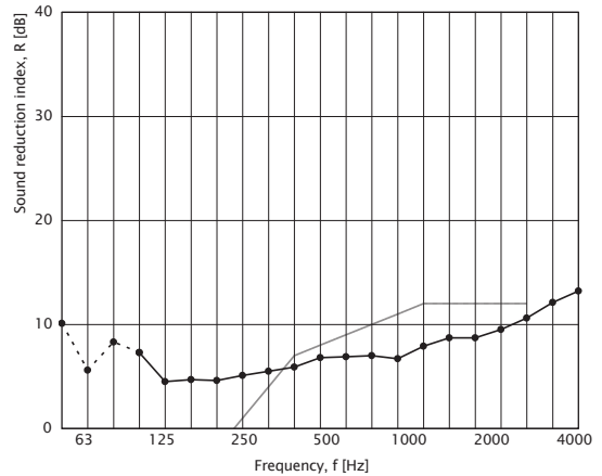
Sound reduction index, R [dB] according to EN/ISO 10140 for 20 mm ISO 120U
